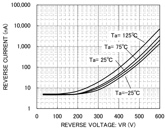
Fig.3 VR-IR CHARACTERISTICS
