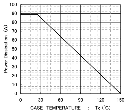
Fig.6 Power Dissipation
