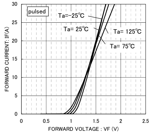
Fig.2 VF-IF CHARACTERISTICS
