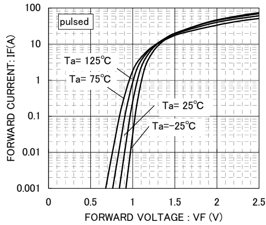
Fig.1 VF-IF CHARACTERISTICS
