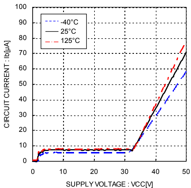
Figure 15. Quiescent current
