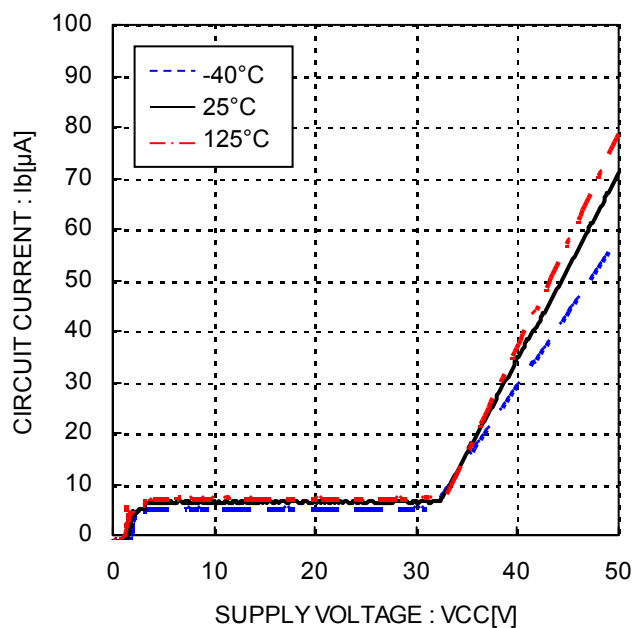
Figure 5. Quiescent current
