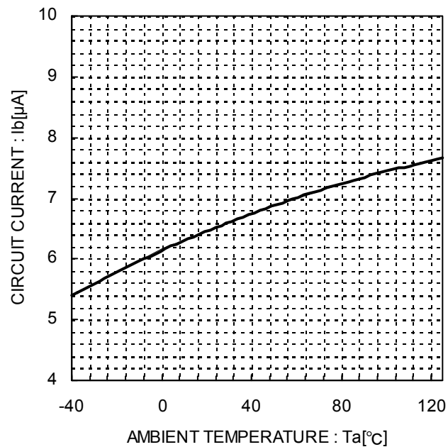
Figure 24. Quiescent current vs. temperature
