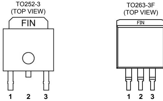
Figure 3. Pin Configuration
