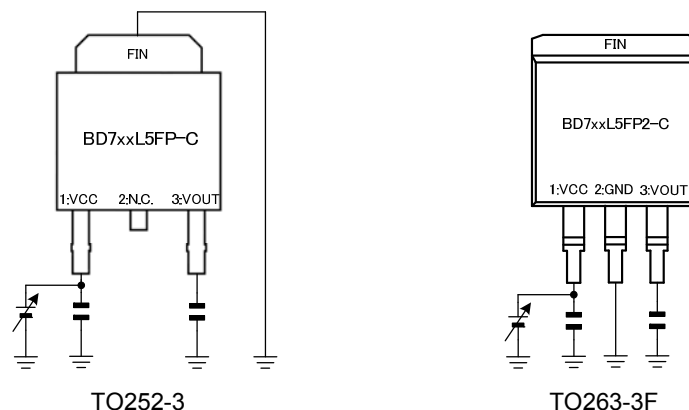
Figure 2. Typical Application Circuits
