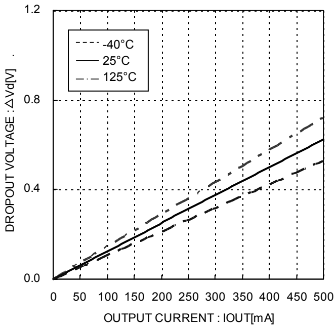
Figure 19. Dropout voltage
