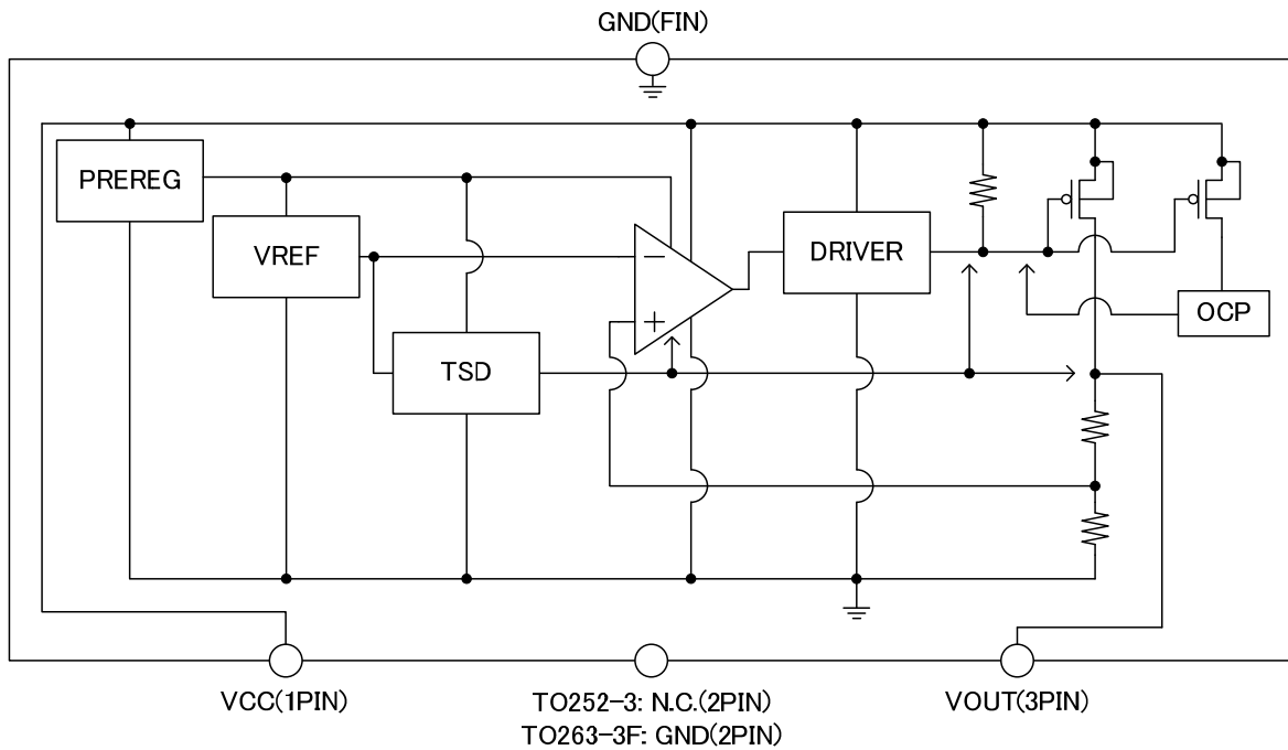
Figure 4. Block Diagram
