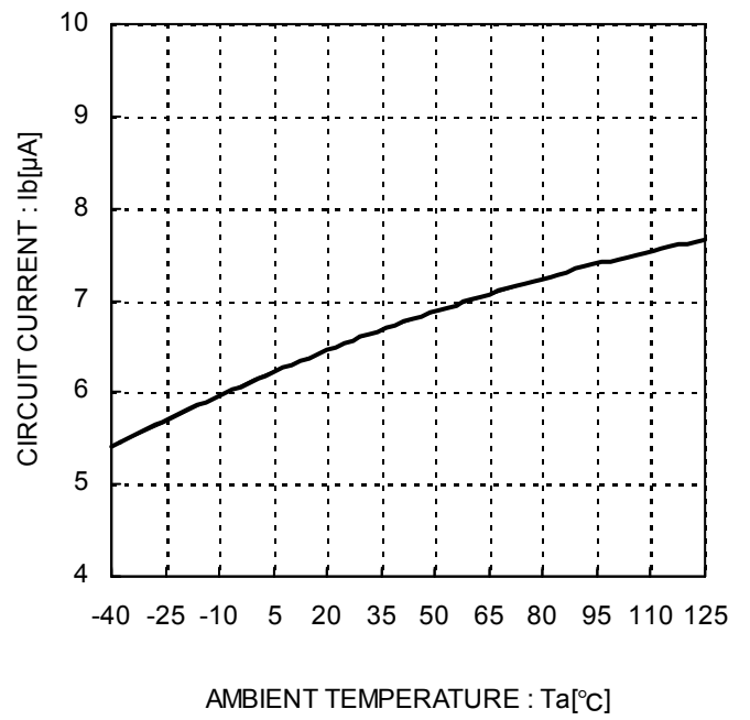
Figure 24. Quiescent current vs. temperature
