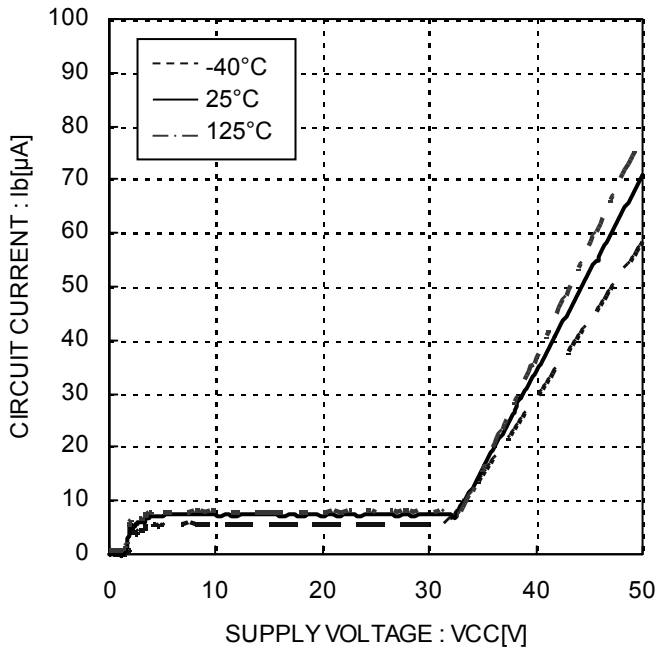
Figure 15. Quiescent current
