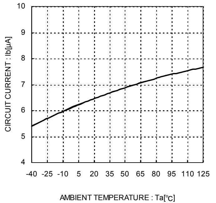
Figure 14. Quiescent current vs. temperature
