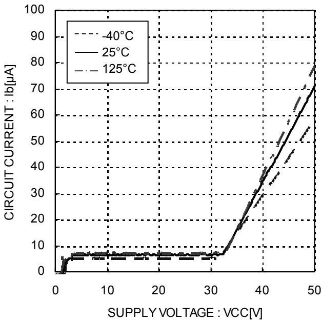
Figure 5. Quiescent current
