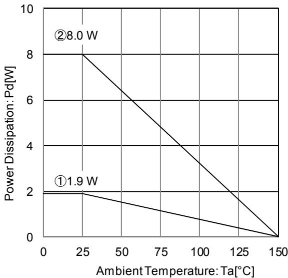
Figure 26. Package Data (TO263-3F)
