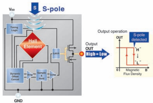
Figure 9a. ROHM Unipolar Hall IC topology shown for S-Pole Detection
