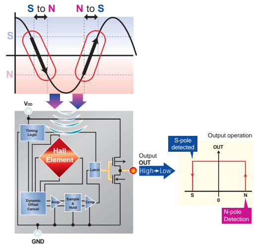
Figure 9d. ROHM Bipolar Hall IC changes state only when magnetic polarity is reversed
