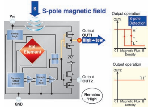
Figure 9c. ROHM Polarity-Discriminating Omnipolar Hall IC Switches have dual outputs
