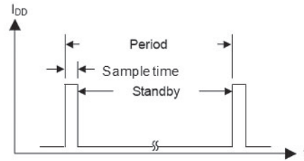
Figure 7. The typical sample time of 48 \mu s for each 50 ms period reduces the average current draw to 8 \mu A or even 5 \mu A.
