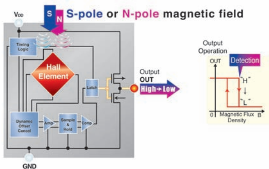
Figure 9b. ROHM Omnipolar Hall IC topology detects either N or S-pole
