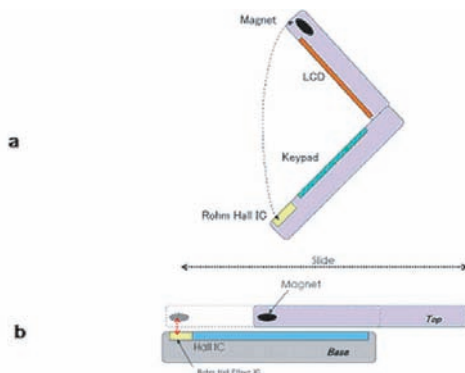
Figure 2. Hall IC switch detects presence of magnet when the phone cover is closed
